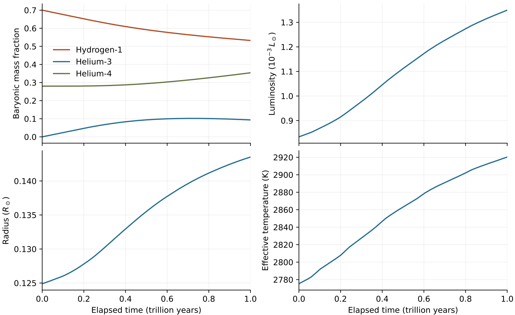
0.1 solar mass: first trillion years of the specified main-sequence model 2048 points · SFII/SVH · COND with convective composition correction
