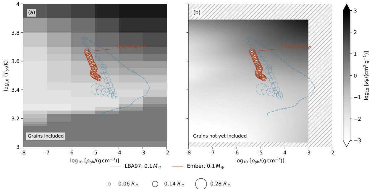
Figure 4: Photospheric evolution of a 0.1M_{\odot} star over hydrogen-rich opacity maps: (a) the grain-inclusive LBA97 Figure 6 map on an approximate calibrated opacity scale; (b) the Rosseland absorption mean of Ember’s SYNPEC wavelength table at X = 0.7 , Z = 0.02 and zero ^3\text{He} . Both panels use identical axes and grayscale normalization. The right map excludes scattering and grains; the low-temperature grain-opacity band in the left map is therefore absent. Hatching marks missing wavelength-table coverage. Both panels show the LBA97 track recovered from 897 figure markers and Ember’s calculated track through 3.848Tyr. The LBA97 curve includes contraction and cooling; the plotted Ember models are burning hydrogen. Open-circle diameters scale with radius, with 48 LBA97 and 22 Ember samples. LBA97 radii are normalized using its stated main-sequence luminosity and temperature. Ember’s local photospheric temperature and density are interpolated at Rosseland optical depth 2/3 using the evolving surface composition. The fixed backgrounds do not represent the changing opacity of either star.
