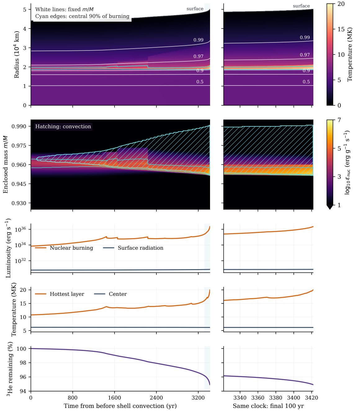
Figure 9: Internal development of the helium-3 pulse on the 666-point grid. The left column spans the computed interval; the right enlarges its final 100 yr on the same clock. Upper panel: temperature versus radius, with white curves following fixed enclosed mass fractions and cyan curves bounding the central 90% of nuclear power. Second panel: specific nuclear heating versus enclosed mass, with connected convective regions hatched. Lower panels show luminosities, temperatures and remaining helium-3. Time zero is an already-burning model before shell convection. The sequence ends during a renewed rise; the final peak and shutdown remain undetermined. The spatial sensitivity is shown in Figure 8.
