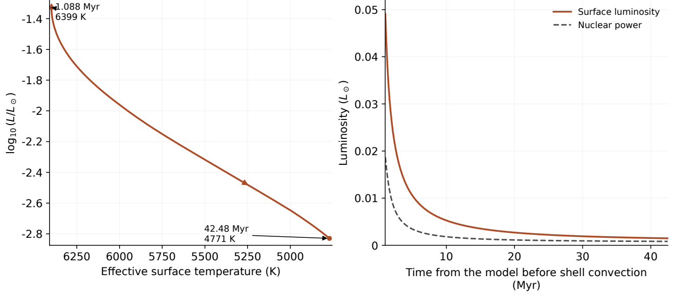
Figure 7: The late shell-burning calculation on 2115 mass points. Left: an enlarged HR diagram around the effective-temperature maximum. The arrow follows increasing time. Right: photon luminosity and deposited nuclear power over the same interval. Time is measured from the model before shell convection. Temperature declines from 6399 K to 4771 K over 4.139 \times 10^7 yr; nuclear burning supplies 55.85% of the final surface luminosity. The contracting model has turned toward cooling. Its physical connection to the calculation resolving the flash from its onset remains unverified.
