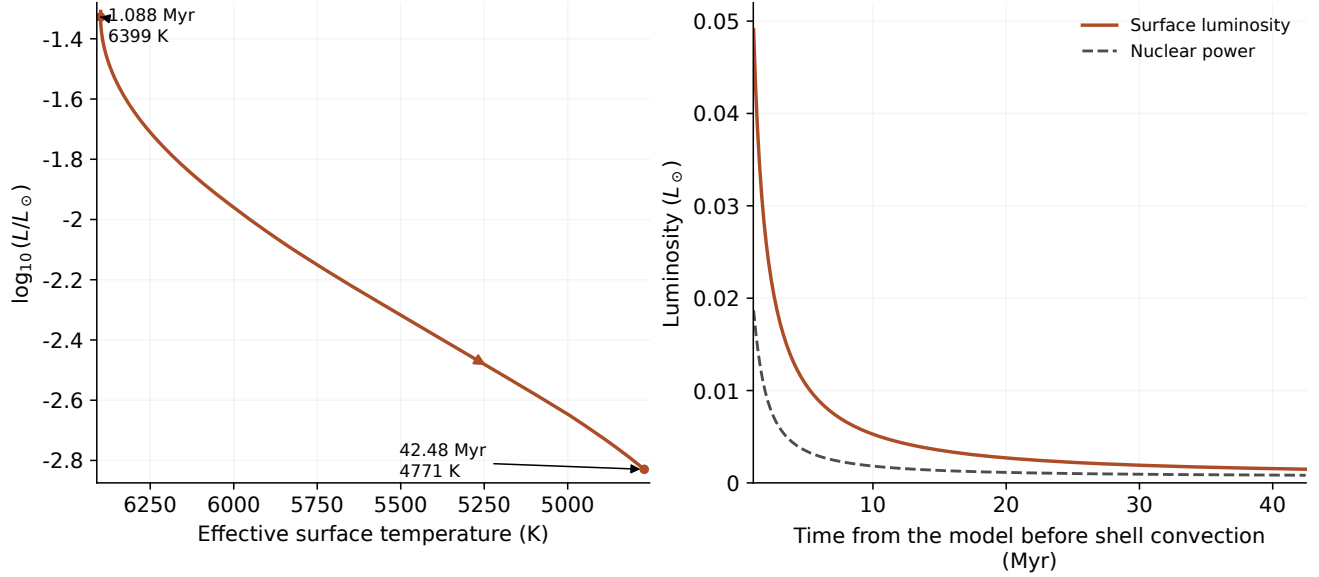
Figure 6: The late shell-burning calculation on 2115 mass points. Left: an enlarged HR diagram around the effective-temperature maximum. The arrow follows increasing time. Right: photon luminosity and deposited nuclear power over the same interval. Time is measured from the model before shell convection. Temperature declines from 6399 K to 4771 K over 4.139 \times 10^7 yr; nuclear burning supplies 55.85% of the final surface luminosity. The contracting model has turned toward cooling. Its physical connection to the calculation resolving the flash from its onset remains unverified.
