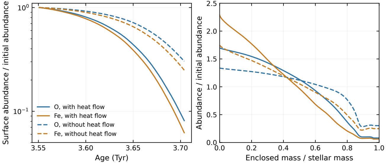
Figure 8: Passive oxygen and iron redistribution on prescribed stellar structures. Left: surface abundance relative to its initial value. Right: the abundance profile at 3.704 Tyr. Solid curves include classical heat flow; dashed curves suppress it. Each tracer’s total inventory is conserved, and the changing convective envelope is mixed by mass. The two heat-flow treatments do not define an uncertainty band, and neither includes the star’s response to the changing metal opacity.
