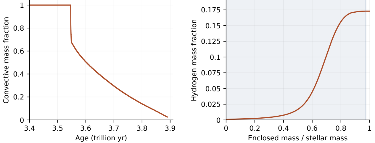
Figure 3: Convection and chemical separation along the Ember track. Left: the fraction of mass in convective regions declines from unity near 3.546Tyr to 0.02565 at 3.890Tyr. Right: the hydrogen profile in the 3.890Tyr model. The shaded core carries heat by radiation and conduction; the outer convective envelope has an almost uniform hydrogen abundance. Both panels use the same calculation and its final saved structure.
