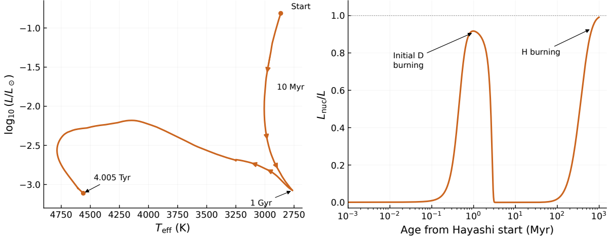
Figure 1: Continuous evolution of the 0.1M_{\odot} model from the Hayashi track. Left: the HR trajectory through 4.005Tyr; arrows show increasing age. Right: nuclear power divided by surface luminosity during the first Gyr; the early maximum is deuterium burning. Age is measured from the contracting starting model. These panels use the same continuous calculation, whose outer boundary remains at optical depth 100. Tracks S, F and P have their own initial models and clocks.
