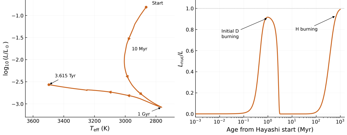
Figure 1: Continuous evolution of the 0.1M_{\odot} model from the Hayashi track. Left: the HR trajectory through 3.615 Tyr; arrows show increasing age. Right: nuclear power divided by surface luminosity during the first Gyr; the early maximum is deuterium burning. Age is measured from the contracting starting model. These panels use the same continuous calculation, whose outer boundary remains at optical depth 100. Tracks S, F and P have their own initial models and clocks.
