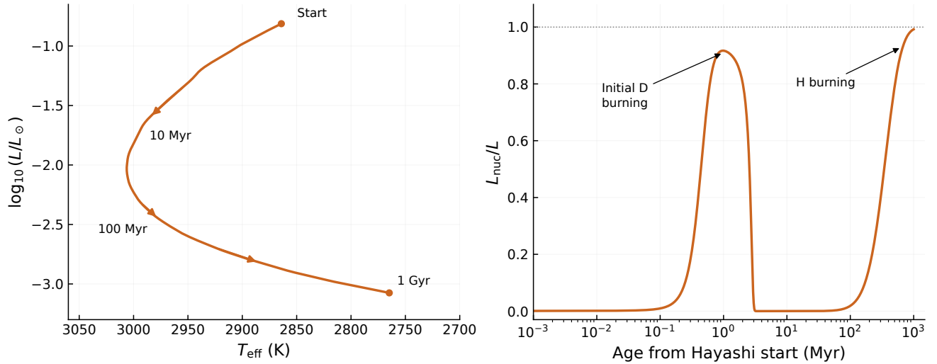
Figure 17: Contraction of the 0.1 M_{\odot} model into the main sequence. Left: the HR trajectory, with arrows indicating increasing age. Right: the fraction of the surface luminosity supplied by nuclear burning. The early maximum is initial-deuterium burning; the later increase is sustained proton–proton burning. At 1 Gyr nuclear power supplies 99.23% of the surface luminosity. Age is measured from the contracting seed. This calculation includes homogeneous convective mixing and initial D/pp burning; it does not include the microscopic element separation or explicit carbon/nitrogen network of the long-term calculations. The curves therefore are not joined to the remnant tracks.
