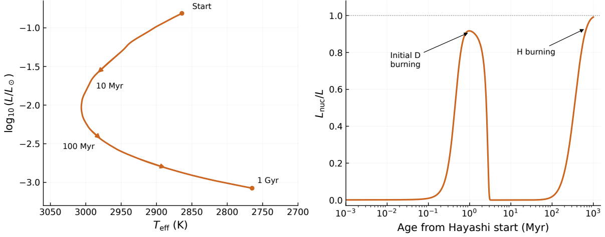
Figure 1: Contraction of the 0.1M_{\odot} model into the main sequence, computed with the continuous driver. Left: the HR track, arrows showing increasing age. Right: the fraction of the surface luminosity supplied by nuclear burning; the early maximum is deuterium burning. Age is measured from the contracting starting model. The plotted sequence ends at 1 Gyr; the same calculation continues to 4 Gyr and, with the composition-dependent atmosphere, to 2.102Tyr (text). It is not joined to Tracks S, F and P.
