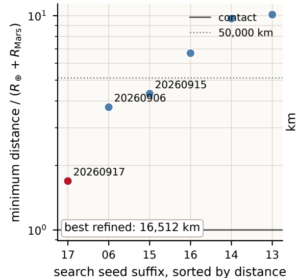
Refined Earth--Mars candidates
