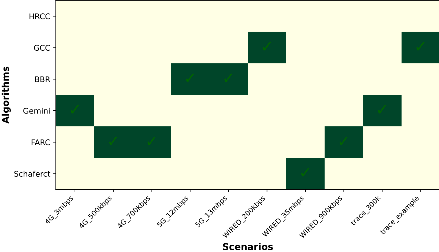
Best Algorithm by Scenario Matrix
