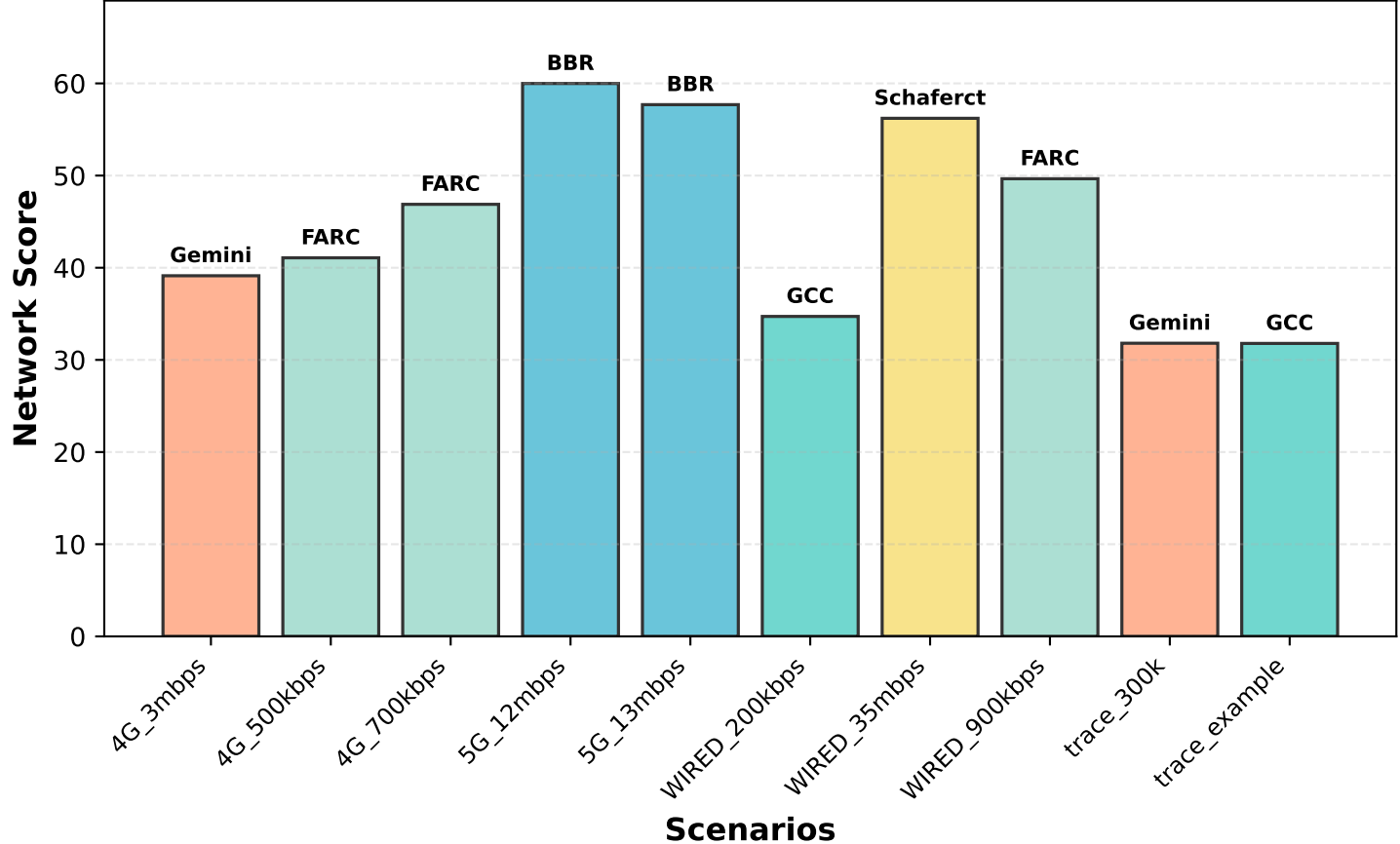
Overall Algorithm Performance
