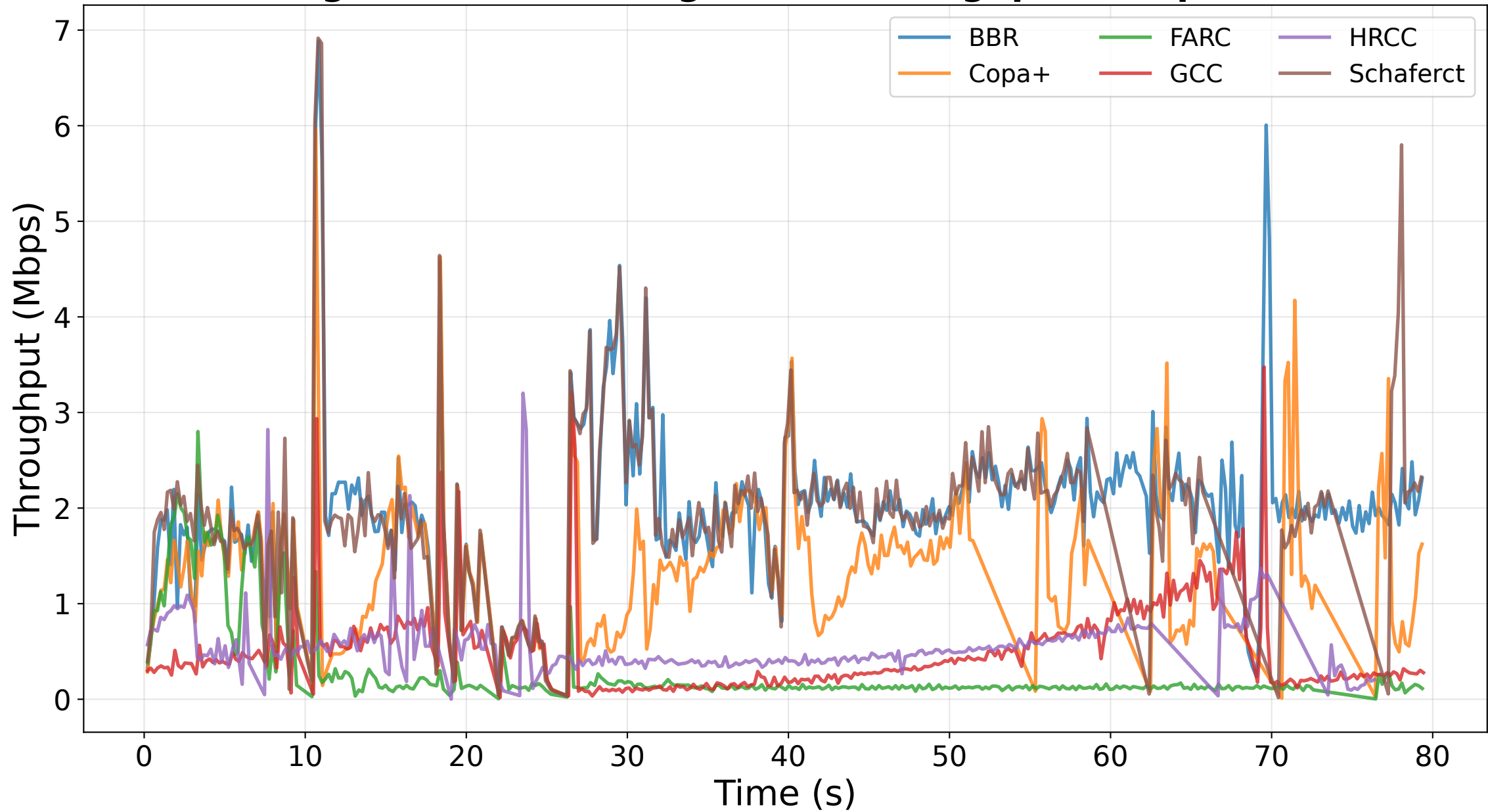
Congestion Control Algorithm Throughput Comparison
