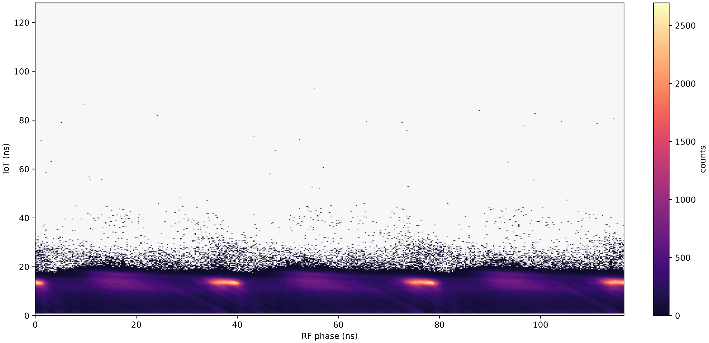
ToT vs RF phase | 3x period | Ch02 | linear Z
