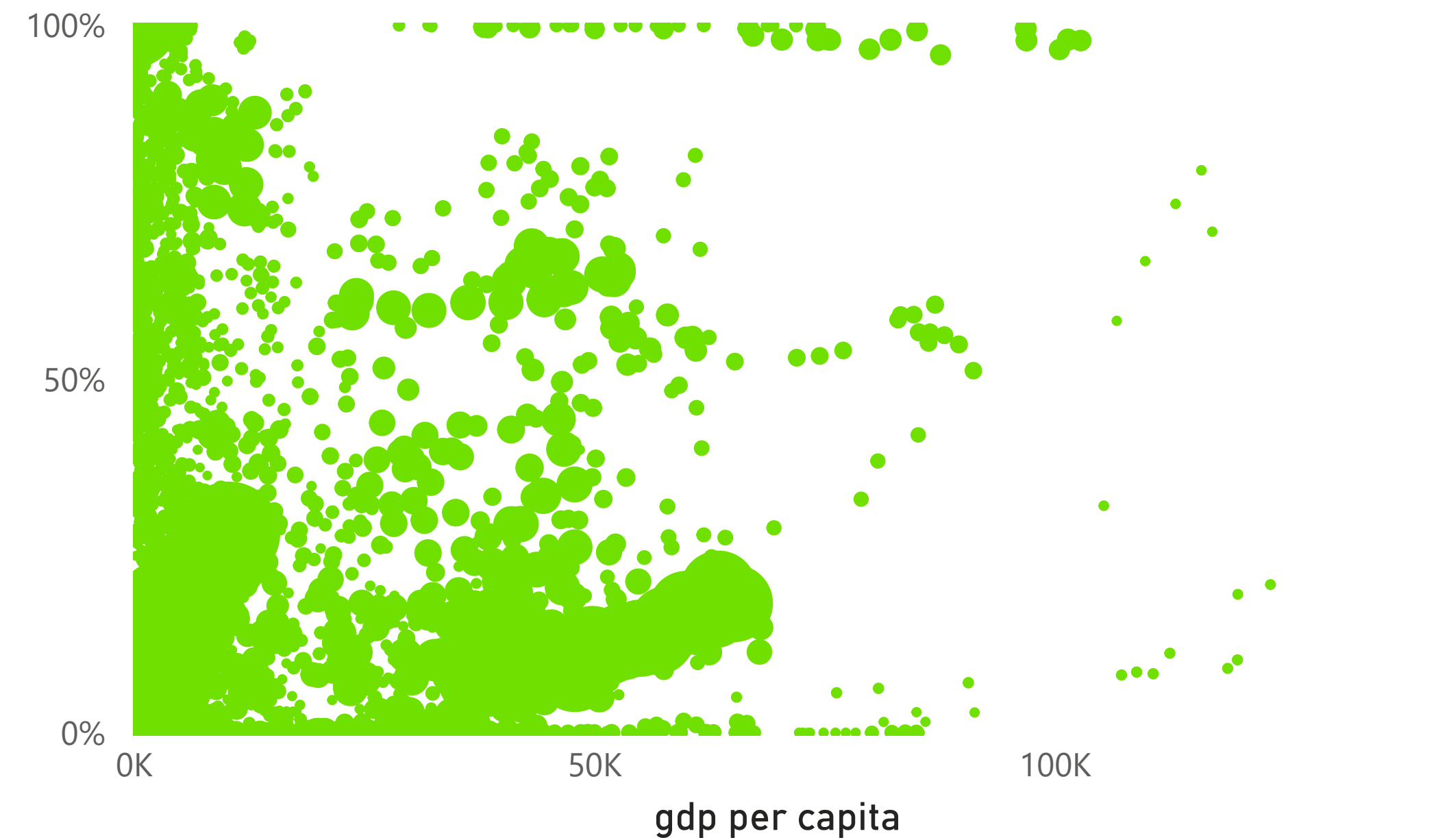
Renewable Share (%) and Total Electricity (TWh) by gdp per capita
