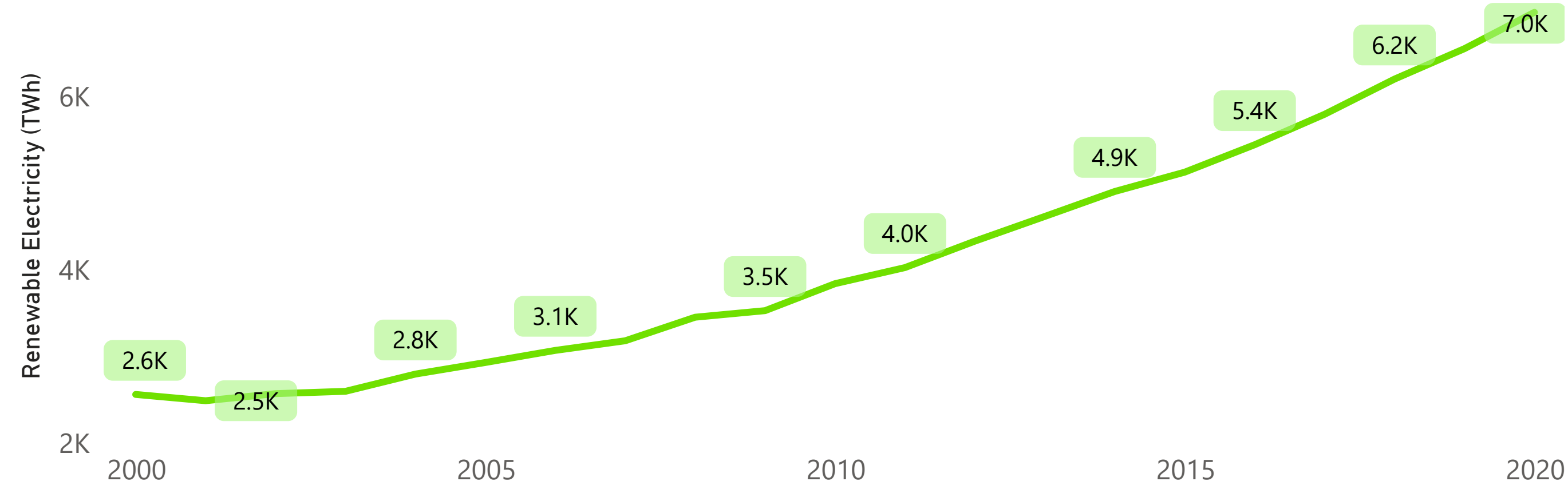
Renewable Electricity utility (TWh) over the Years
