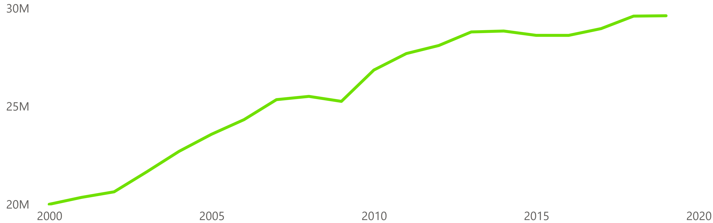
Total CO2 Emissions (kt) by Years
