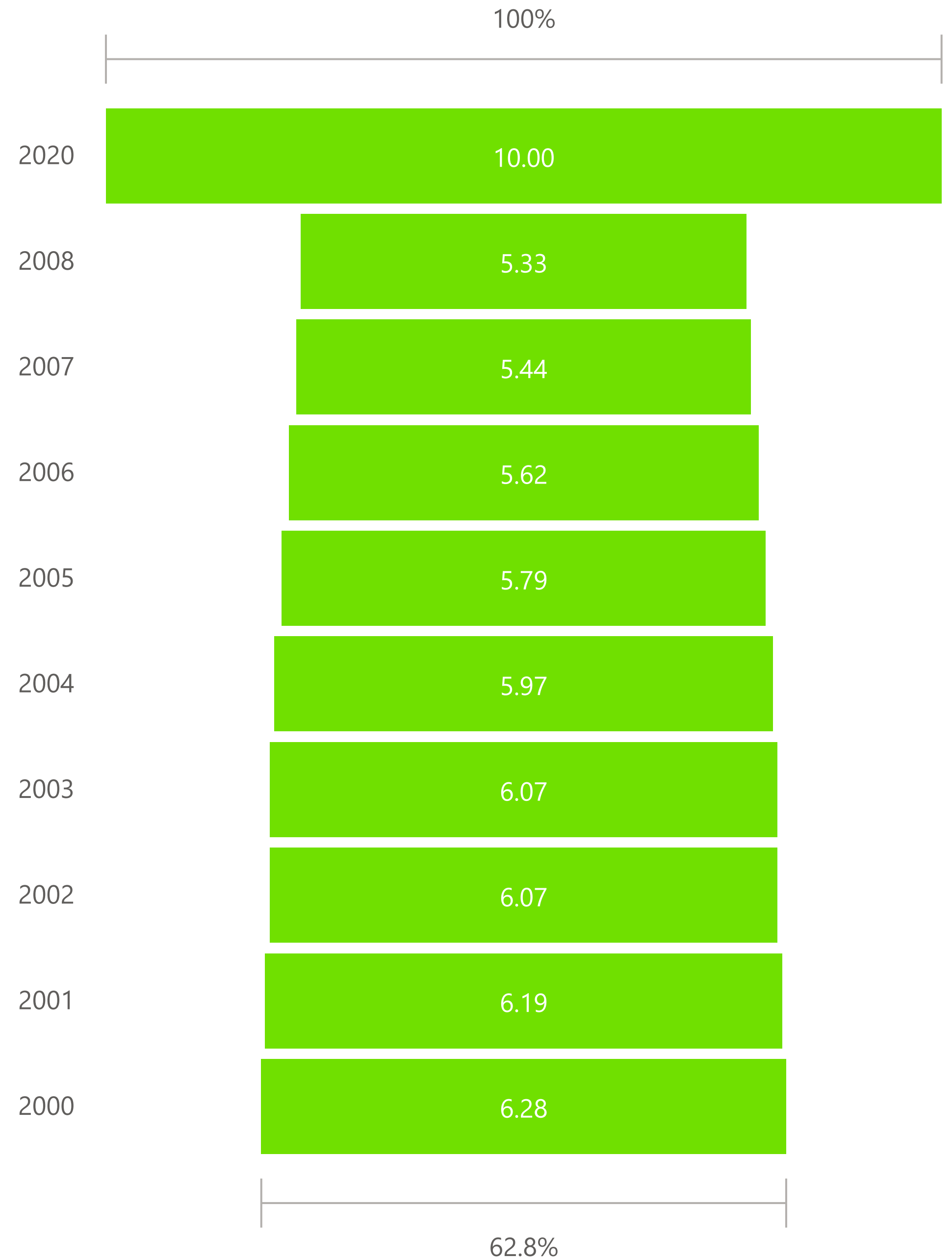
Avg Energy Intensity by Year
