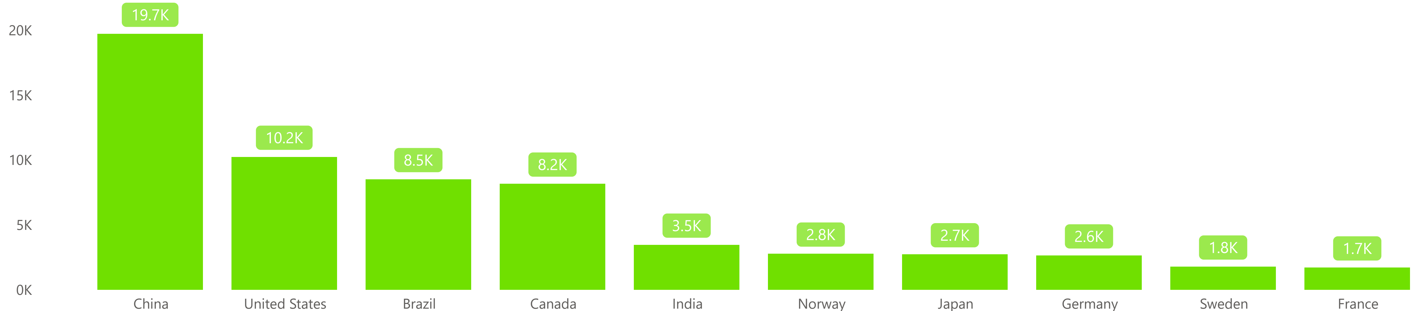
Renewable Electricity (TWh) by Countries
