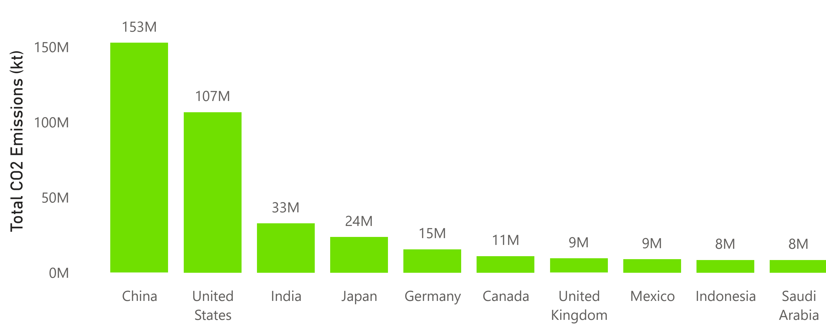
Total CO2 Emissions (kt) by Entity
