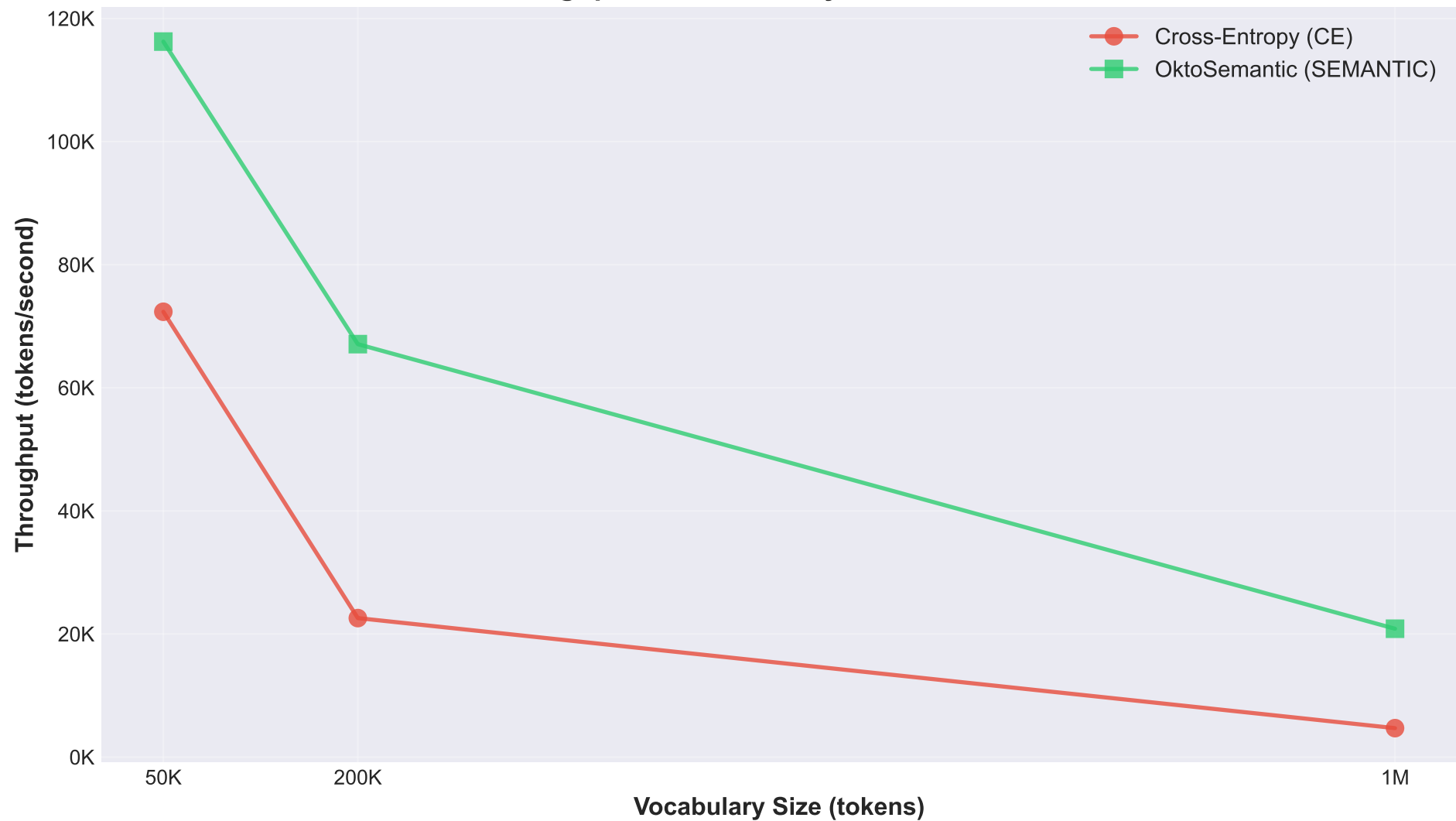
Throughput vs Vocabulary Size - RTX A6000
