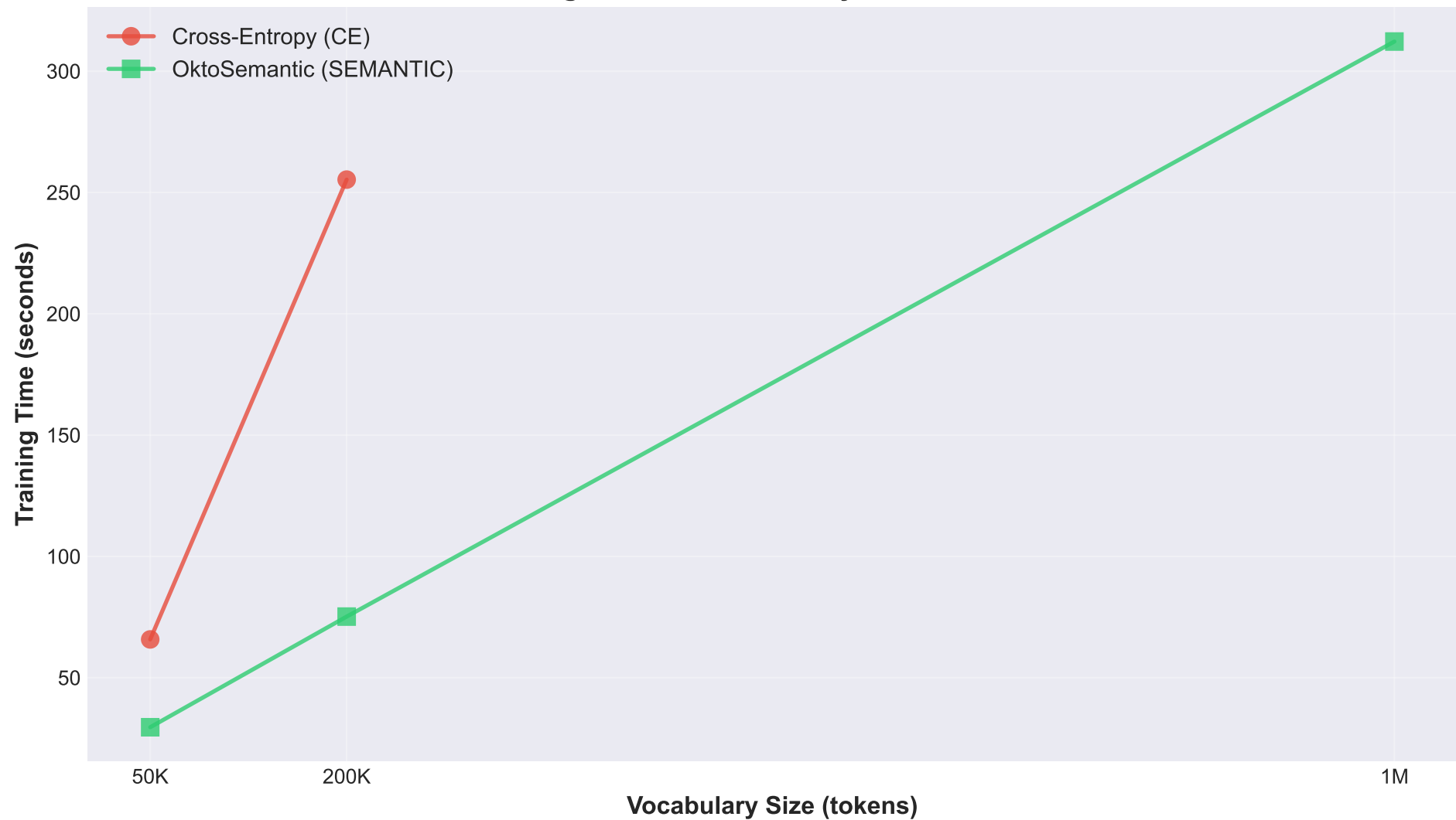
Training Time vs Vocabulary Size - RTX 4070
