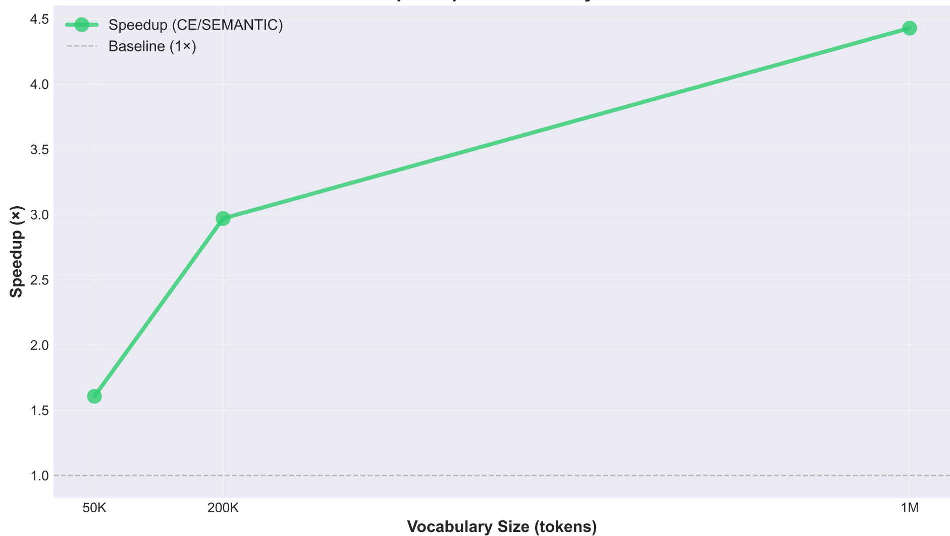
OktoSemantic Speedup vs Vocabulary Size - RTX A6000
