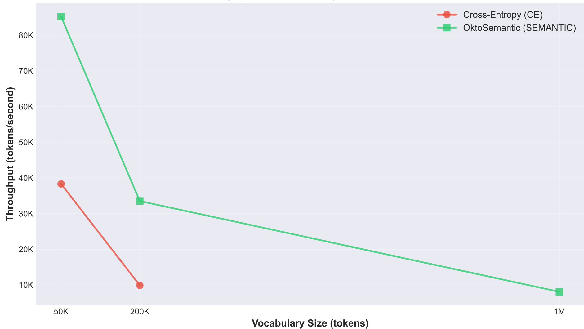
Throughput vs Vocabulary Size - RTX 4070
