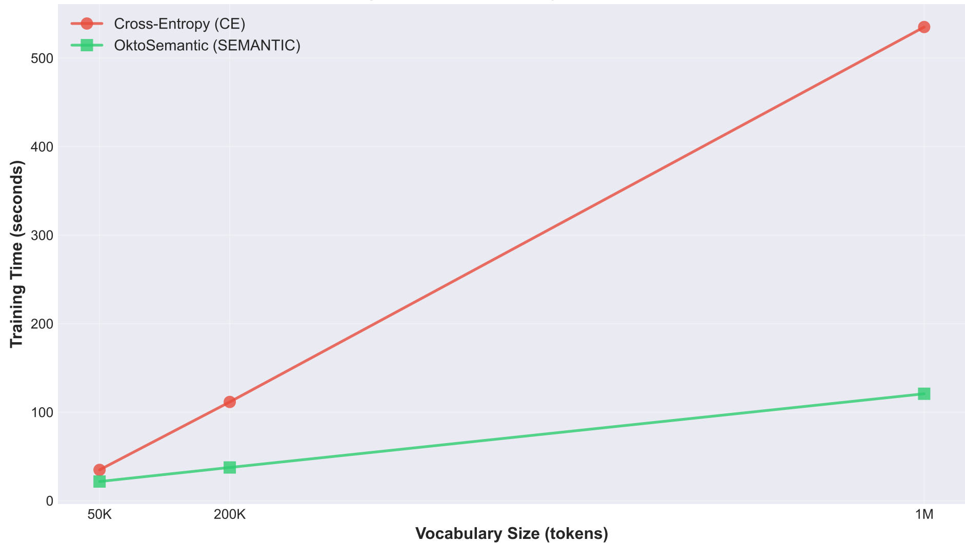
Training Time vs Vocabulary Size - RTX A6000
