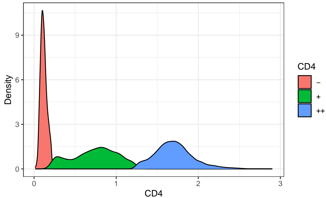
CD4 CLR distribution with GMM clustering
