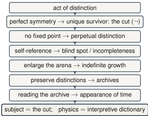
The argument as a single descending chain.
