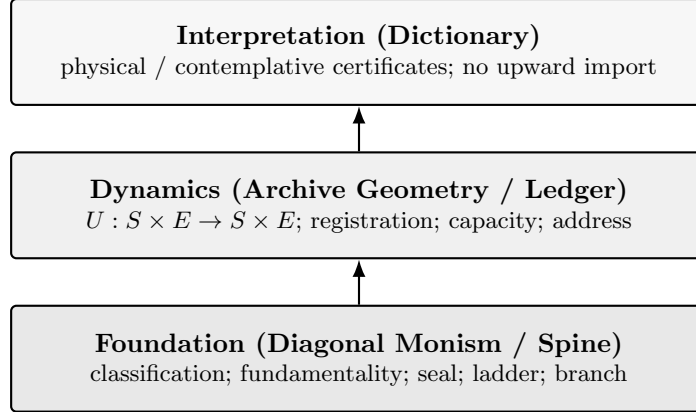
Figure 1: Three-layer architecture. Arrows indicate permitted dependence (foundation supports dynamics; dynamics support interpretation). The figure orients the reader; it proves nothing.
