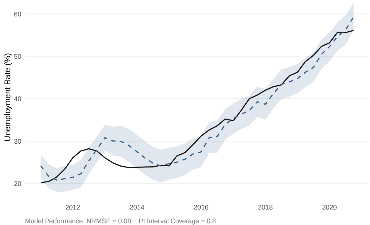
Figure 5: Rolling Out-of-Sample Reconstruction
