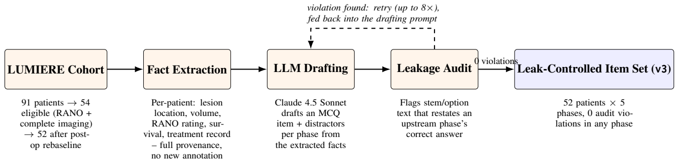
Figure 2: Construction pipeline for the leak-controlled (v3) LUMIERE item set. Structured per-patient facts are extracted from LUMIERE, an LLM drafts multiple-choice items from those facts, and an automatic auditor flags any item that restates an upstream phase’s correct answer, feeding violations back into the drafting prompt for up to eight retries.
