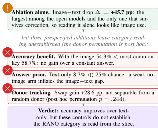
Figure 3: Worked example (Llama-4-Scout, DSCR): the ablation drop, largest among the open models and surviving correction, would alone credit image use, but the three prespecified additions (accuracy benefit over the answer prior, the prior itself, and donor tracking, the last a post hoc permutation) do not establish that the category is read from the slice.
