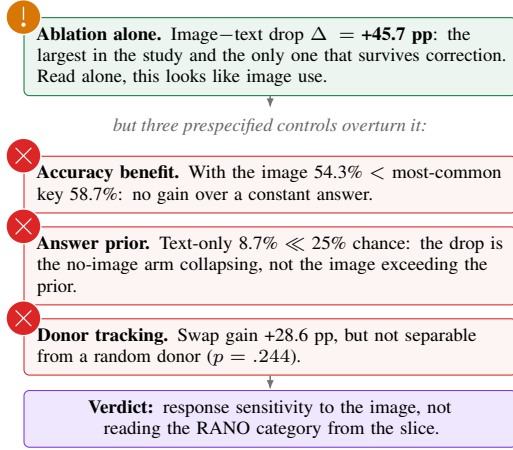
Figure 3: Worked example (Llama-4-Scout, DSCR): the ablation drop is the largest in the study and survives correction, so reading it alone would credit image use, but the three prespecified additions (accuracy benefit over the answer prior, the prior itself, and donor tracking) do not support that reading.
