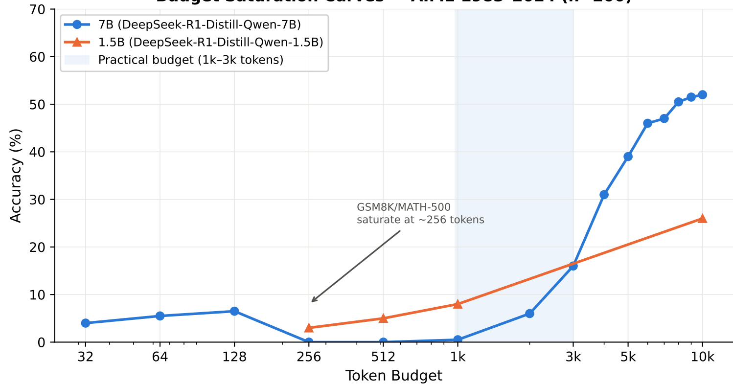
Budget Saturation Curves — AIME 1983-2024 (n=200)
