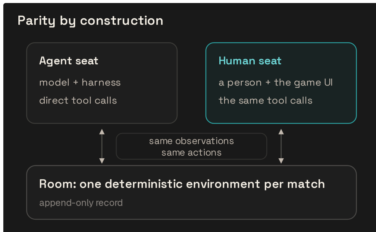
Figure 7. Only the interface layer differs between a human seat and an agent seat.
