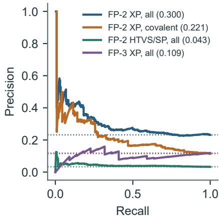
B Precision-recall
