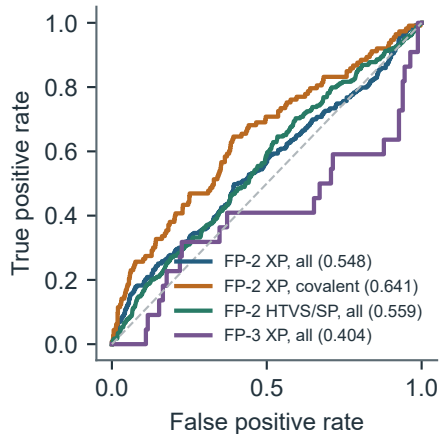
A ROC
