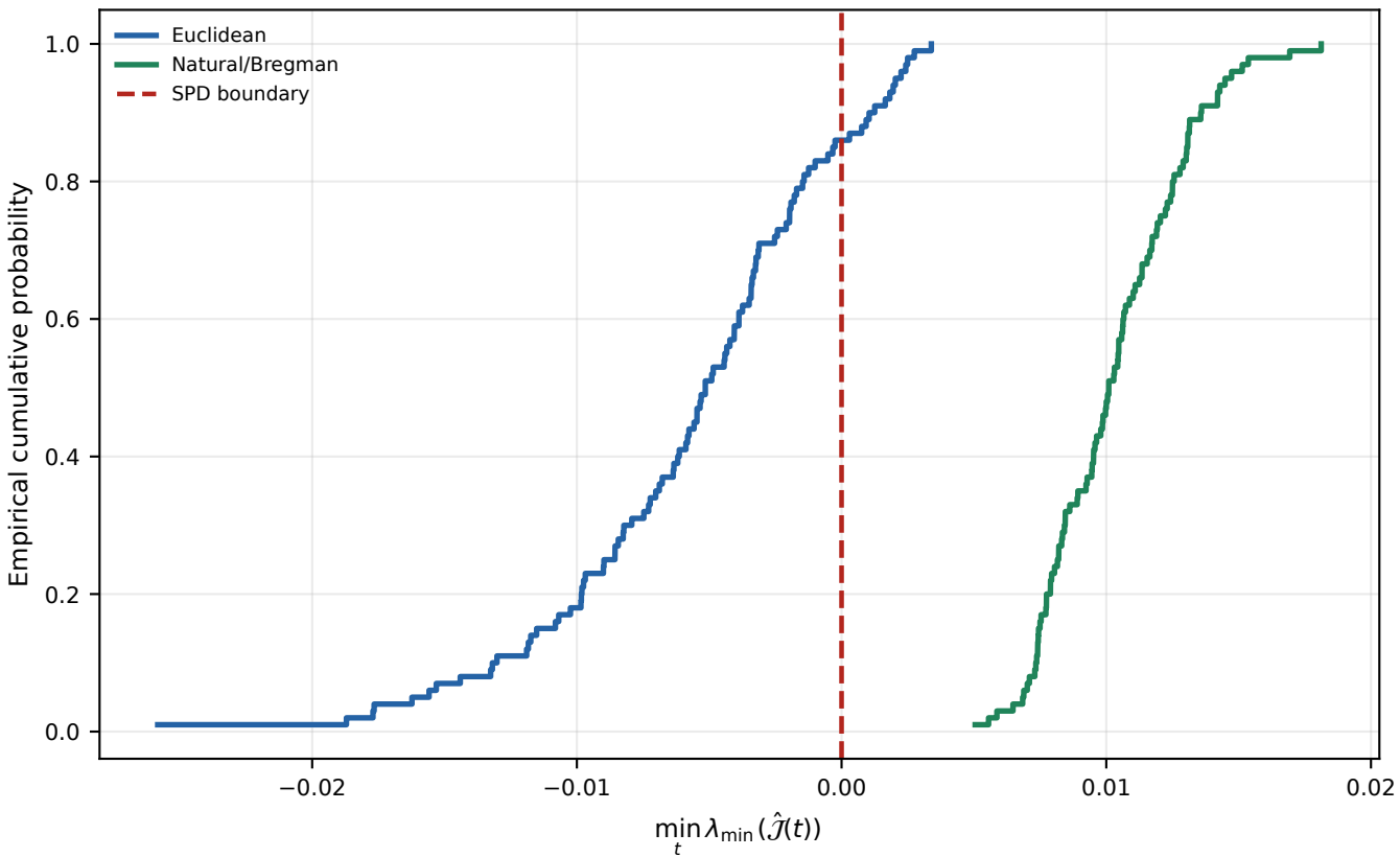
Physical-consistency margins
