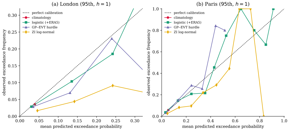
Figure 2: Reliability diagrams for the exceedance probability at the 95th percentile ( h=1 ) for (a) London and (b) Paris. In both cities the logistic regression and the GP-EVT hurdle track the diagonal (calibrated) and spread their predictions (informative); the zero-inflated log-normal is systematically overconfident (its predicted exceedance probabilities exceed the observed frequencies), despite attaining nominal conformal coverage by construction. Climatology is a single point at the base rate.
