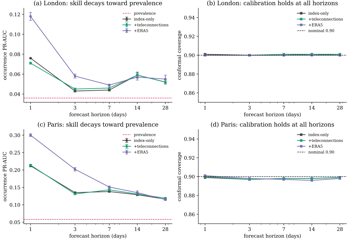
Figure 4: Seed-averaged horizon sweep on the 95th-percentile index (GP-EVT hurdle) for both cities: (a,b) London, (c,d) Paris. (a,c) Occurrence PR-AUC decays toward the prevalence floor (dashed) as the forecast horizon grows; the +ERA5 driver gain is clearest at h = 1 and fades into seed noise by h = 3 . (b,d) Conformal coverage stays at the nominal 0.90 across all horizons and predictor sets. Error bars / markers are means over three seeds.
