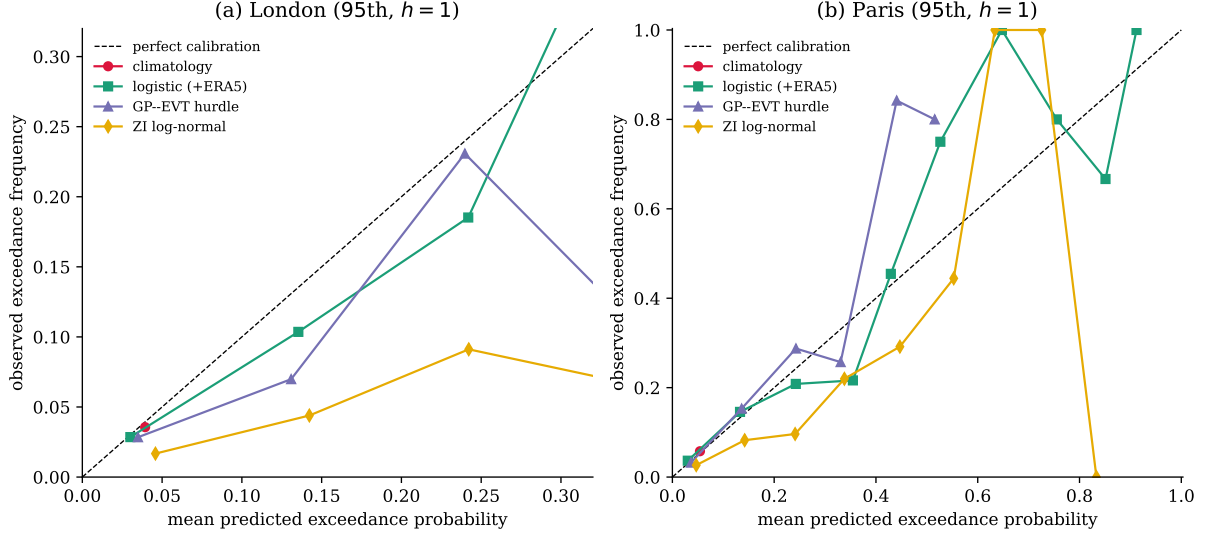
Figure 2: Reliability diagrams for the exceedance probability (95th, h=1 ): (a) London, (b) Paris. In both cities the logistic regression and the GP-EVT hurdle track the diagonal (calibrated) and spread their predictions (informative); the zero-inflated log-normal is systematically overconfident (its predicted exceedance probabilities exceed the observed frequencies), despite attaining nominal conformal coverage by construction. Climatology is a single point at the base rate. (Paris is noisier at high predicted probabilities, where few days fall.)
