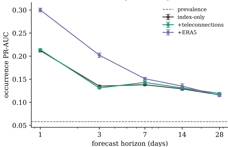
(c) Paris: skill decays toward prevalence
