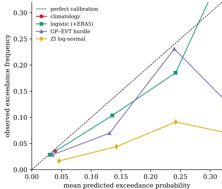
(a) London (95th, h = 1 )
