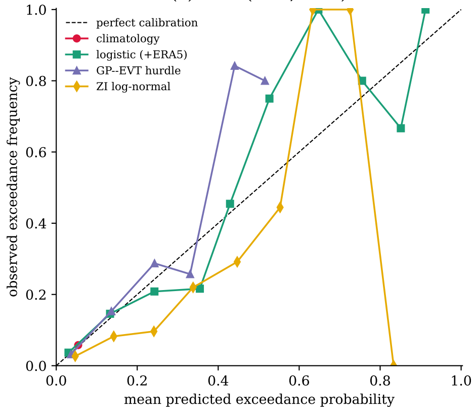
(b) Paris (95th, h = 1 )
