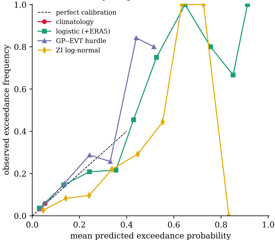
Reliability diagram (Paris 95th, h = 1 )
