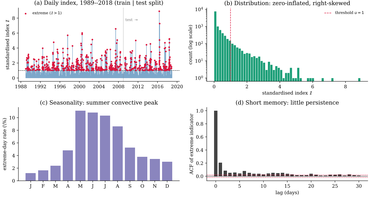
Figure S1: Paris 95th-percentile precipitation-extreme index (Paris counterpart of Figure 1 in the main paper). (a) Daily index with extreme days ( \mathcal{I} > 1 ) and the train|test split; (b) zero-inflated, right-skewed distribution; (c) summer-peaked seasonality of the extreme-day rate; (d) short memory of the extreme indicator.
