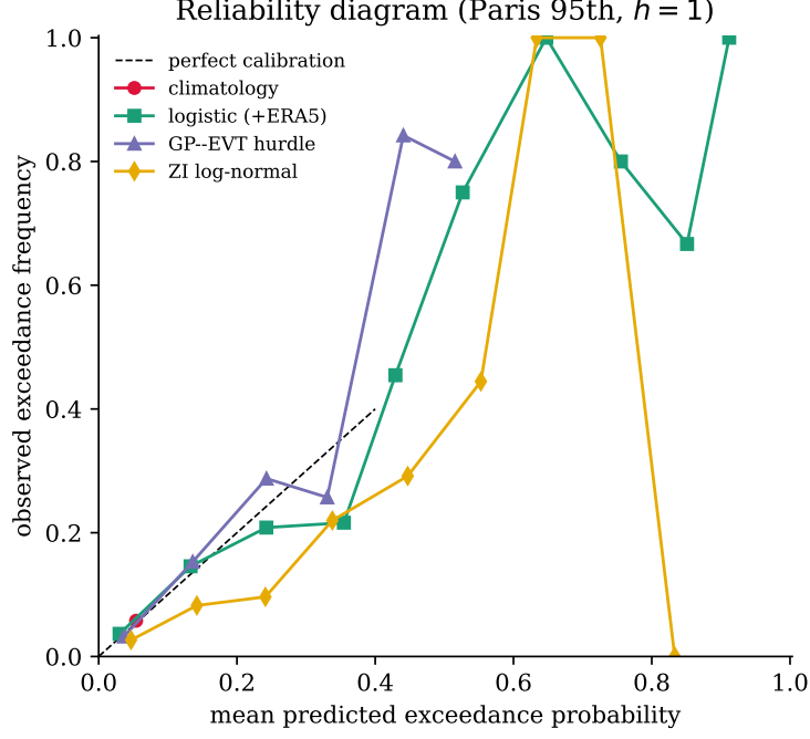
Figure S2: Reliability diagram for the Paris exceedance probability (95th, h = 1 ; Paris counterpart of Figure 2). The calibrated logistic model and the GP-EVT hurdle track the diagonal; the zero-inflated log-normal is systematically overconfident despite attaining nominal conformal coverage, mirroring London.
