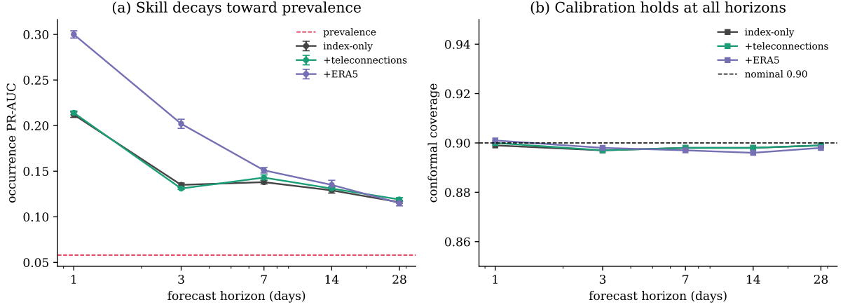
Figure S3: Seed-averaged horizon sweep on the Paris 95th-percentile index (Paris counterpart of Figure 4; GP-EVT hurdle). (a) Occurrence PR-AUC decays toward the prevalence floor (dashed) as the horizon grows, with the +ERA5 gain clearest at h = 1 ; (b) conformal coverage holds at the nominal 0.90 across horizons and predictor sets. Markers are means over three seeds.
