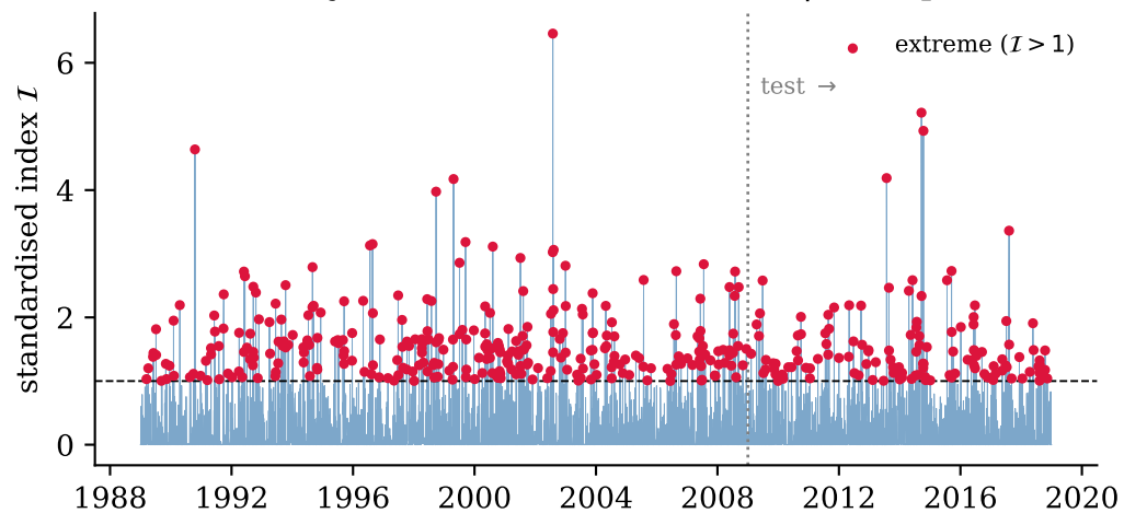
(a) Daily index, 1989--2018 (train | test split)
