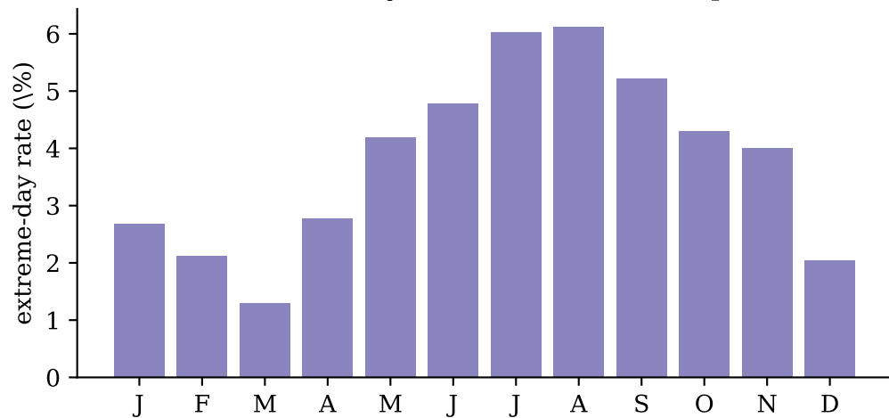
(c) Seasonality: summer convective peak
