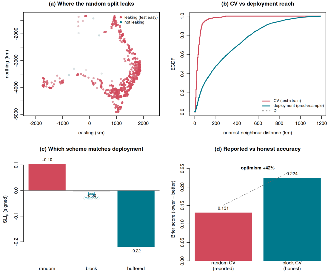
Figure 5: Auditing a species distribution model (south-east Australia presence/absence; Valavi et al., 2019). (a) Per-point leakage map: most test points are easier under random CV than at deployment. (b) The CV nearest-neighbour distances (red) sit far to the left of the deployment distances (blue): test points are much closer to training data than the wall-to-wall map will be ( \phi = variogram range). (c) Signed SLI by candidate scheme—random CV is optimistic, buffered CV is over-corrected into pessimism, block CV best matches deployment. (d) Consequence: the Brier score reported under random CV (0.131) is 42% better than the honest, design-matched value (0.224).
