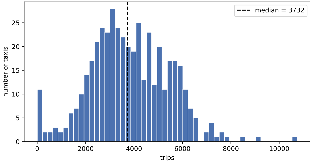
Trips per taxi (448 taxis)
