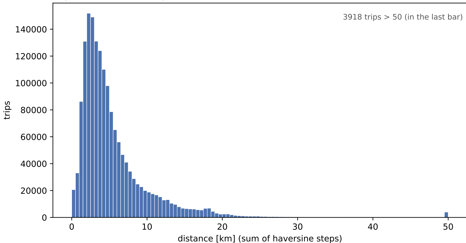
Trip distance (valid trips)
