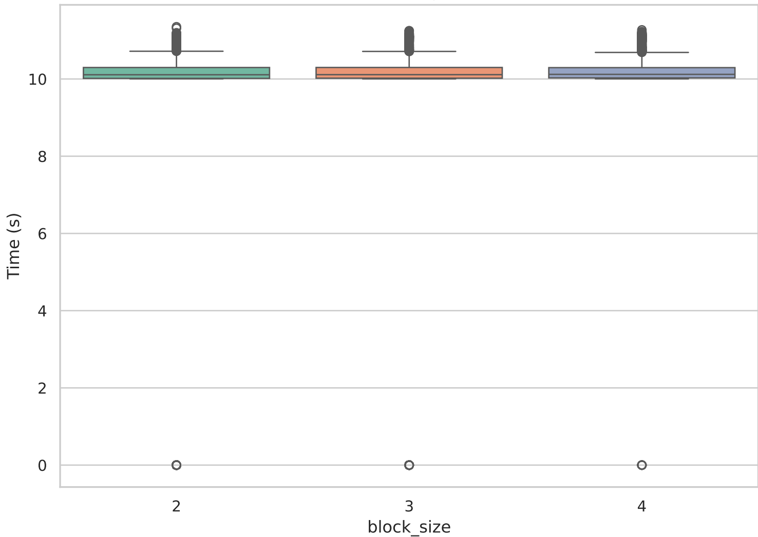
Wall-clock Time by Block Size
