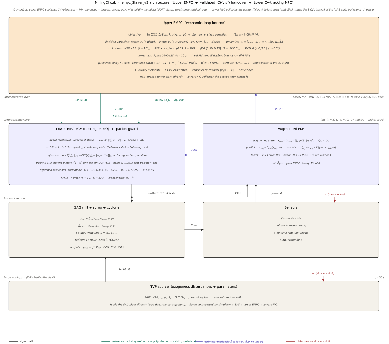
Figure 2. The two-layer EMPC control architecture: the upper EMPC (economic, long horizon) publishes a validated reference packet (CV*, u*) through a packet guard to the lower CV-tracking MIMO MPC; an augmented EKF estimates the mill and sump states plus the ore-hardness parameter, and a disturbance/parameter (TVP) source drives the simulated plant.
