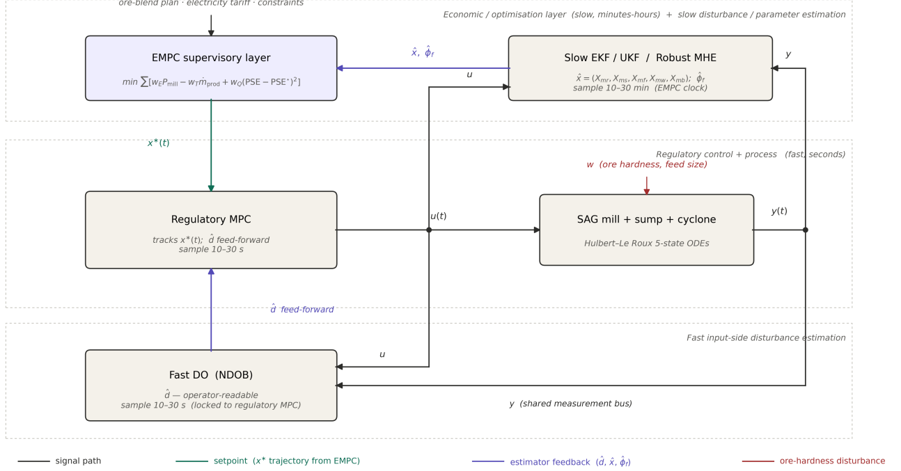
Figure 3.2 — Two-time-scale observer stack for the proposed SAG-mill EMPC. Top tier (slow, 10–30 min, EMPC clock): EMPC supervisory layer (left) and the Slow EKF/UKF / Robust MHE (right) which delivers \hat{x} and the slowly-drifting parameter \hat{\phi}_f to the EMPC. Middle tier (fast, 10–30 s): regulatory MPC and the Hulbert–Le Roux SAG plant. Bottom tier: Fast DO (NDOB), locked to the regulatory MPC clock, supplying \hat{d} as feed-forward. Black signal lines carry plant input u(t) and measurement y(t) ; both are tapped to feed both estimators (EKF/UKF/MHE and NDOB are model-based and require u in their prediction step). Teal is the EMPC's reference trajectory x^*(t) to the regulatory MPC. Indigo is estimator feedback ( \hat{d} from DO; \hat{x}, \hat{\phi}_f from EKF/UKF/MHE). Red w is the dominant ore-hardness / feed-size disturbance. Slow \phi_f -drift is absorbed by the EKF/UKF/MHE's integrating-disturbance state rather than a separate mismatch-detector block (cf. Olivier-Craig 2013, Mittermaier et al. 2025).
