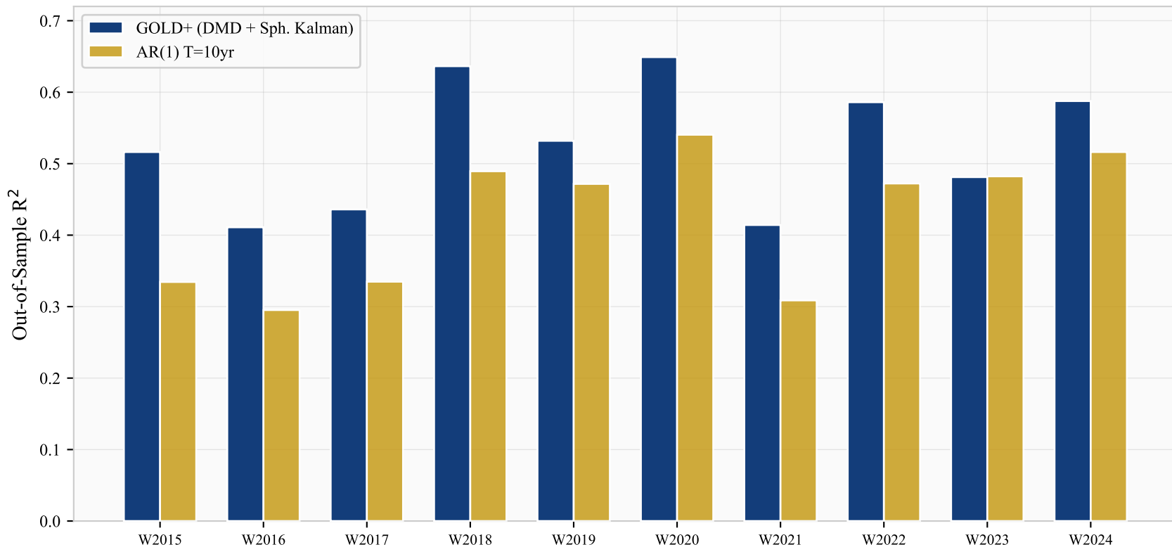
Per-Window Performance: GOLD+ vs AR(1)
