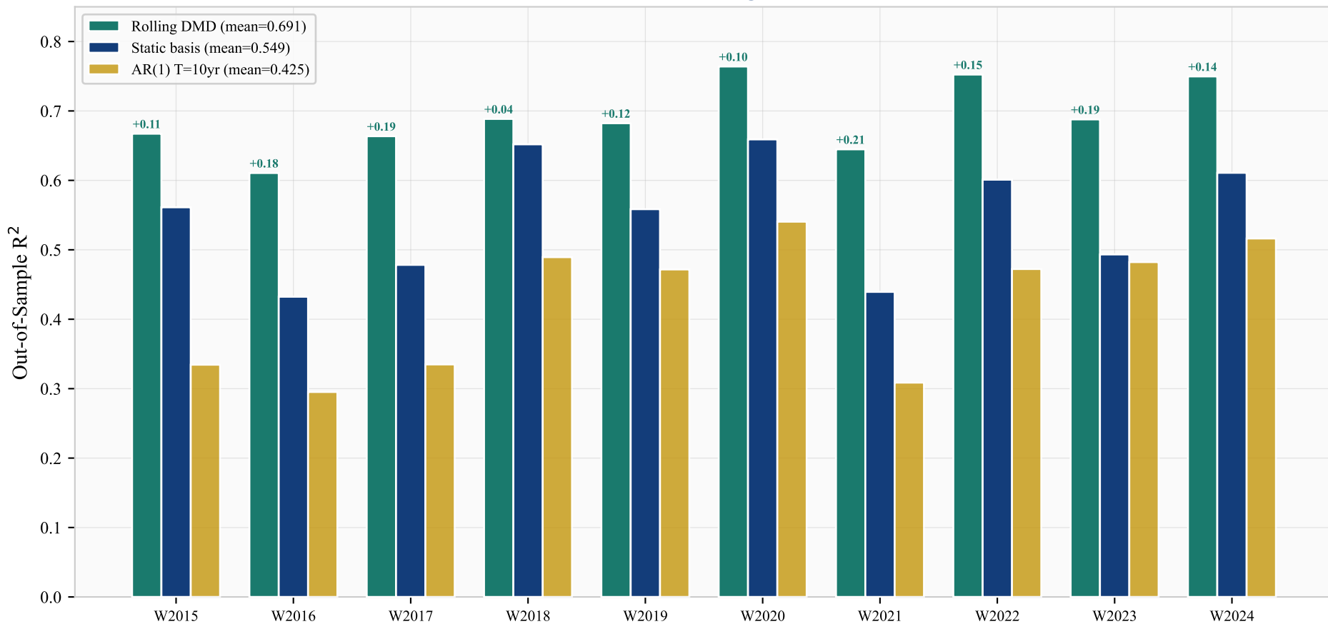
Per-Window Performance: Rolling vs Static Basis vs AR(1)
