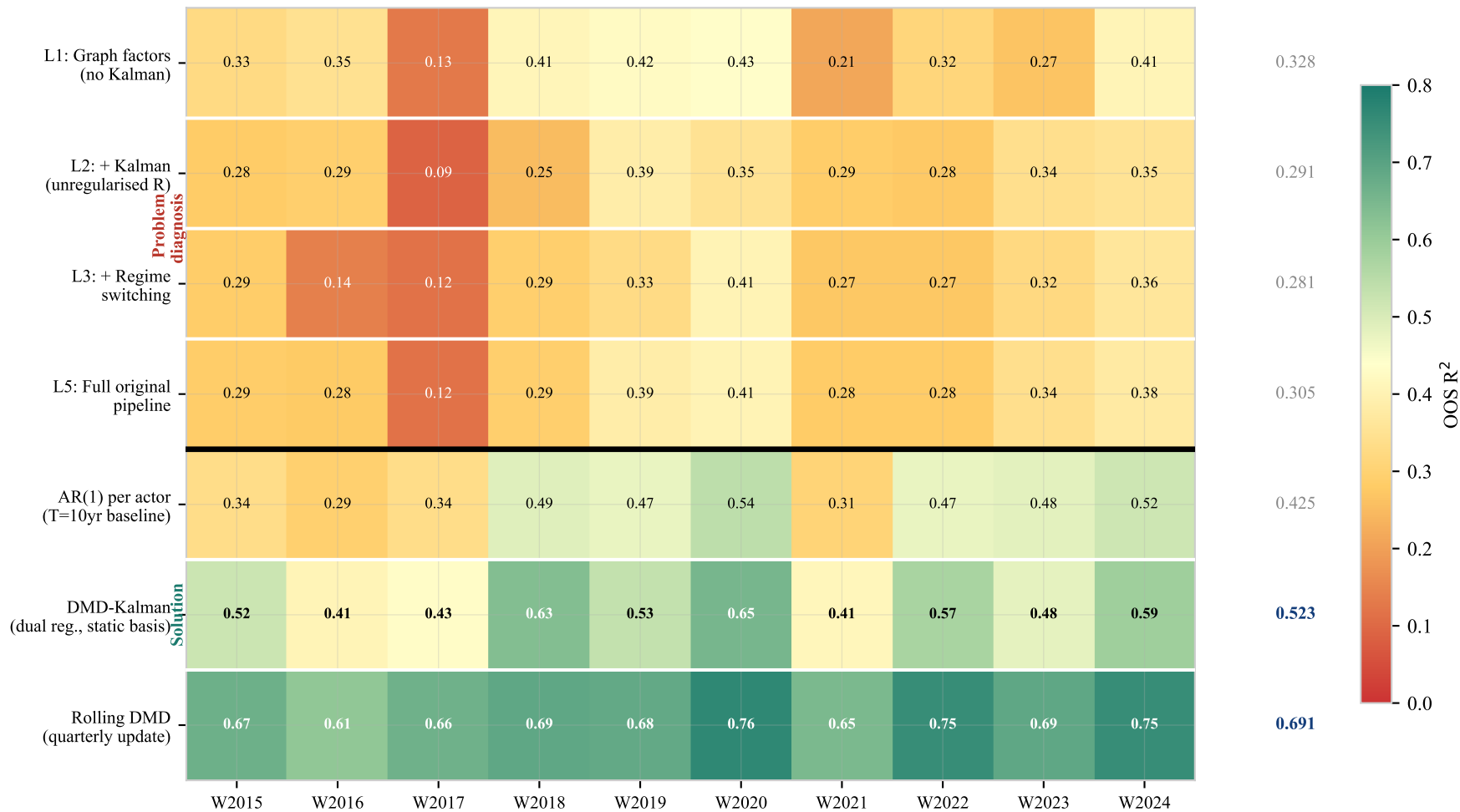
Component Ablation: From Unregularised Kalman to Rolling DMD
