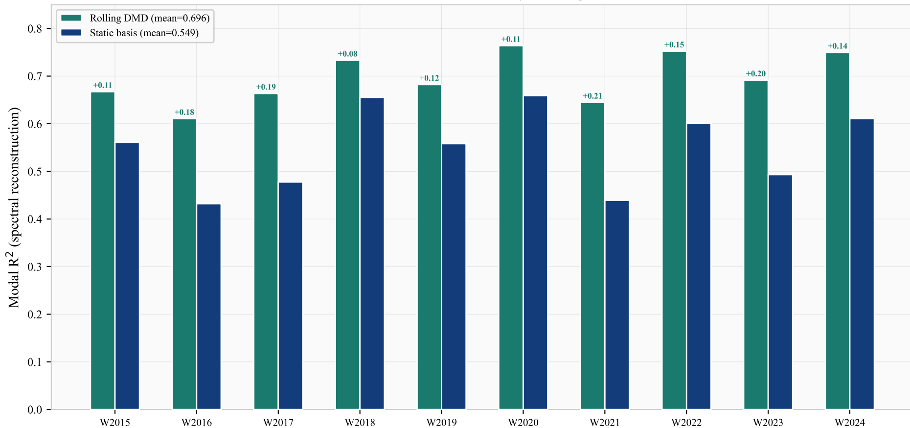
Per-Window Reconstruction Quality: Rolling vs Static Basis
