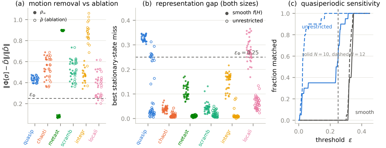
Figure 5: (a) Coherence removal on both channels, all N=10 runs: the motion-removal channel \rho_\infty = \sum_E P_E \rho P_E (filled) versus the stronger full-diagonalization ablation \bar{\rho} (rings). For the metastable and integrable classes the two differ decisively — most of their registered “jump” was deletion of stationary degenerate structure — while the nondegenerately-supported classes coincide. Removing exactly the motion still changes the metric in every class. (b) The smooth-in-energy representation gap: best miss found, \|\Phi[\sigma] - \bar{D}\|/\|\bar{D}\| per run, both sizes pooled, for smooth- f(H) stationary ensembles (filled; \leq 24 parameters) versus unrestricted diagonal-population optimization (rings; 2^N parameters). Only the quasiperiodic class shows a robust, all-run gap between the two; Table 3 completes the family spectrum: the full commutant matches the quasiperiodic metric almost exactly, and the sector control shows at what cost. (c) Threshold sensitivity for the quasiperiodic class: fraction of runs matched versus threshold, per search family and size; the registered \varepsilon_\Phi = 0.25 (vertical line) sits in the steep region of the unrestricted N = 10 curve, so counts at that threshold are sensitive — the smooth/unrestricted gap is not.
