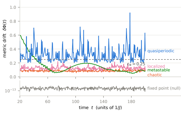
Figure 2: Metric drift \delta\Phi(t) for representative runs ( N = 10 ). The chaotic metric is stationary under the preregistered threshold while the quasiperiodic metric oscillates far above it; the metastable class shows its slow coherent wave; the localized run sits near the threshold (the class straddles it, 80/100 stationary at N = 12 ). Bottom strip: the frozen null at machine precision. Ensemble verdicts are given in the text.
