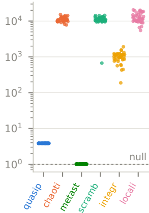
PR_A (Bohr ratio)
