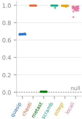
\bar{d} (recurrence mean)
