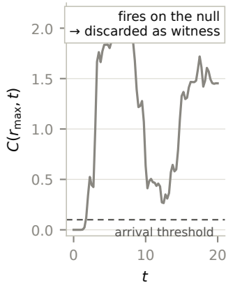
W3 (OTOC) on the frozen null
