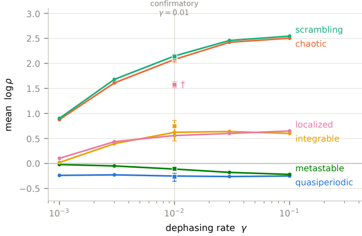
Figure 4: Dephasing response by class: mean \log \rho versus rate \gamma (descriptive sweep, curves; first 10 manifest runs per class, Néel-primary for the localized regime). Squares with intervals: the confirmatory single- \gamma ensemble means with BCa 95% CIs. (†: the confirmatory localized ensemble uses 5 initial states per realization and reads higher than the Néel-primary sweep — an ensemble-composition difference, not a discrepancy.) The sign structure — negative for coherence-carried classes, strongly positive for chaotic ones — is stable over two decades and never reorders.
