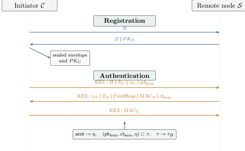
Figure 2: Hybrid PQ-OPAQUE message flow between an initiator and a remote node. ML-KEM public and ciphertext material are carried in KE1 and KE2, while account and transcript binding feed the authenticated key schedule without adding an authentication message.
