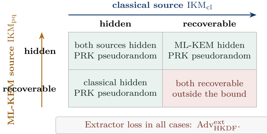
Figure 5: Condition map for the hybrid-combiner interpretation used in Eq. (20). Rows and columns describe whether the classical or ML-KEM source remains hidden relative to a fixed transcript. Under the extractor interpretation, the PRK remains pseudorandom whenever at least one source remains hidden; simultaneous recovery of both sources is the source-level condition not ruled out by the bound, up to the additive extractor term.
