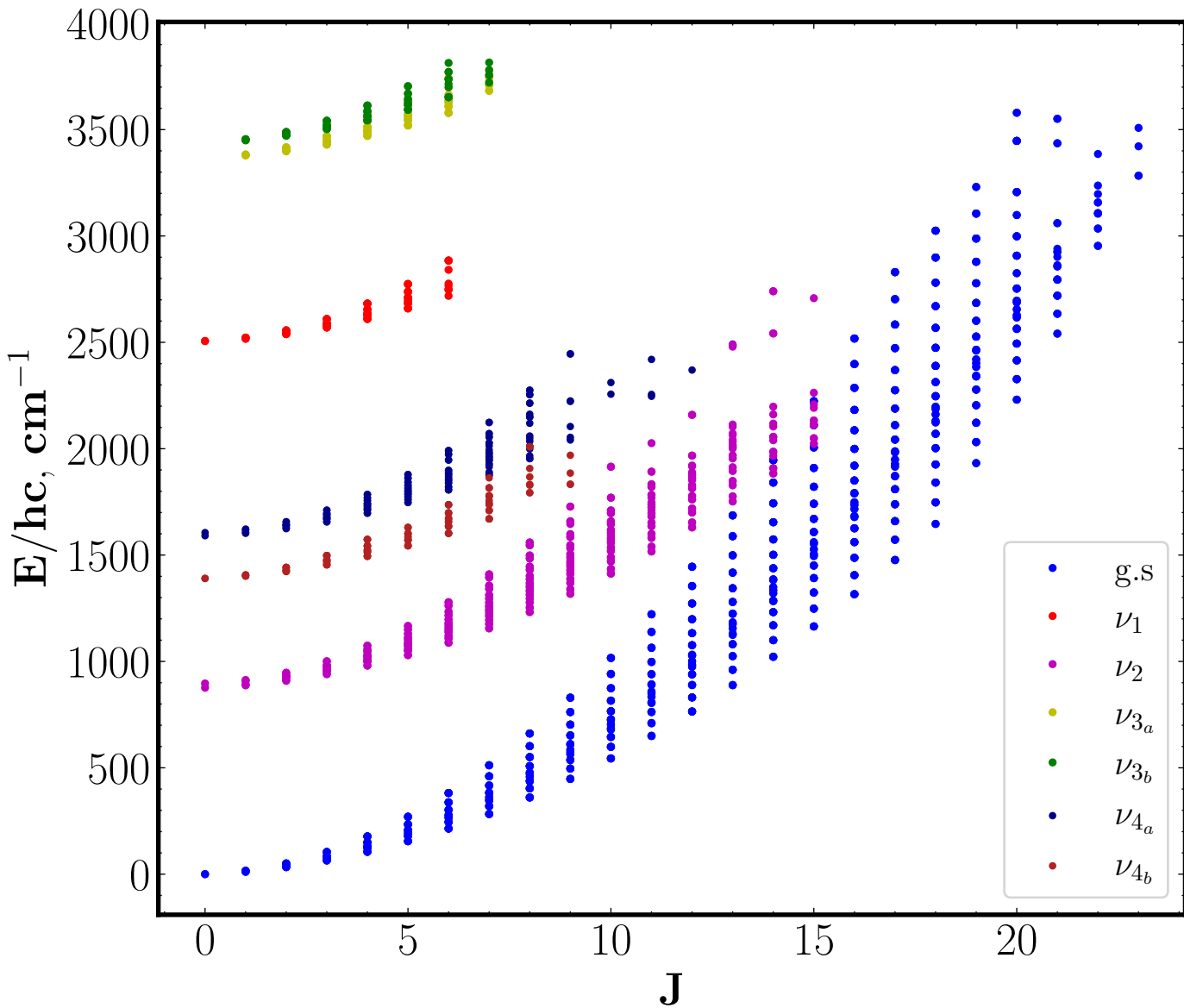
(a) \text{NH}_2\text{D}
