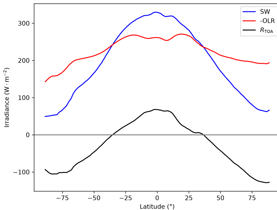
Figure 2.4: Zonal and annual mean average of irradiance from PI control simulations.
